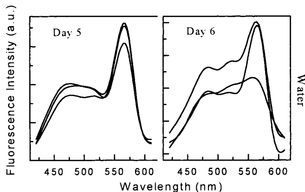
Fig. 7. Measured two-photon fluorescence spectra for group 1 muscle stored in water for 5 or 6 days.
